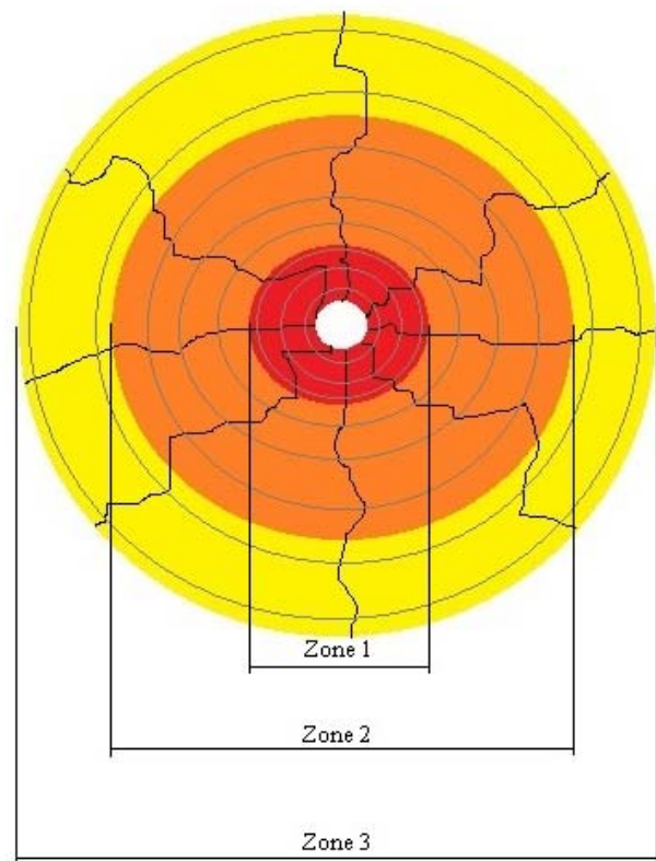
Fig. 1. Various zones arising from hole blasting (red – zone 1, orange – zone 2, yellow – zone 3).
