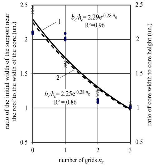
Figure 9. Graph showing dependences of width-to-height ratio of bearing cores (1) on support width (under the roof) to core width (2) on the quantity of partitions n_g in the support ( \times and \blacksquare - markers to trend lines 1 and 2, respectively).
