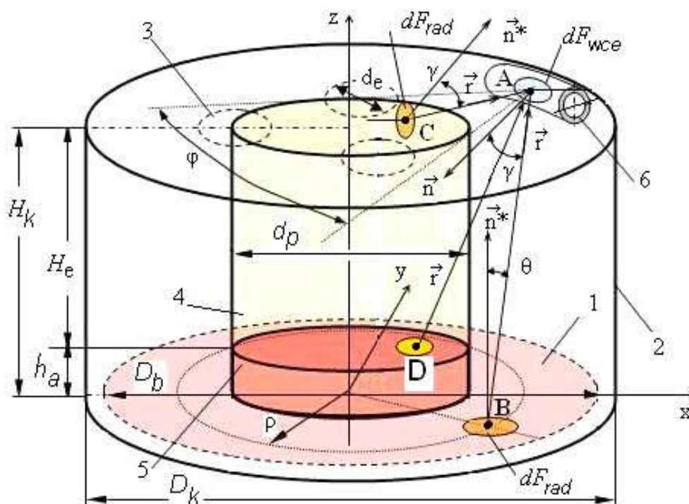
Figure 1 – Scheme of heat exchange by radiation in the EAF workspace. 1 – bath, 2 – casing, 3 – electrode, 4,5 – conditional surfaces of electrodes and arcs, respectively, 6 – WCE x, y, z, ρ – coordinates; γ, θ – direction angles, r – radius-vector
